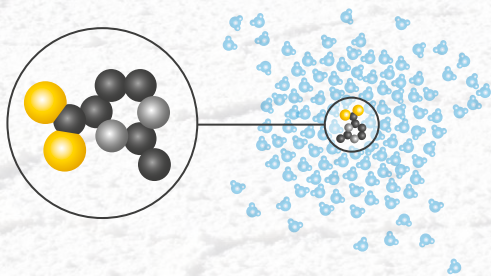
medEctoin® molecule medEctoin®-hydrocomplex
