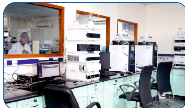
HPLC Area
