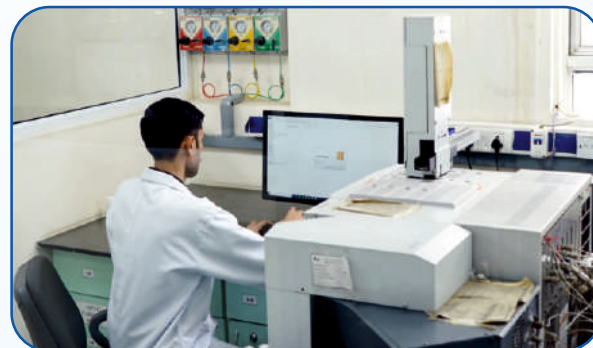
Gas Chromatography
