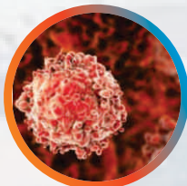
Dasatinib IP
