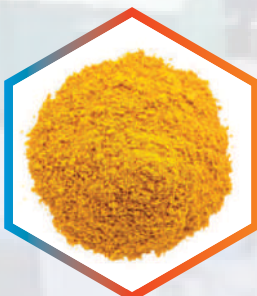
Tetrahydrocurcumin
