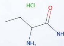
(S)-(+)-2-Aminobutanamide hydrochloride
