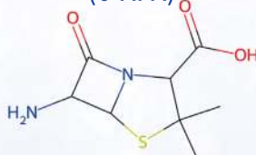
(+)-6-Aminopenicillanic acid (6-APA)
