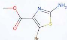
Methyl 2-amino-5-bromothiazole-4-carboxylate
