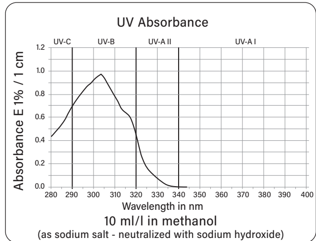
Phenylbenzimidazole Sulfonic Acid
