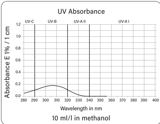
Homosalate
