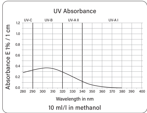
Octocrylene
