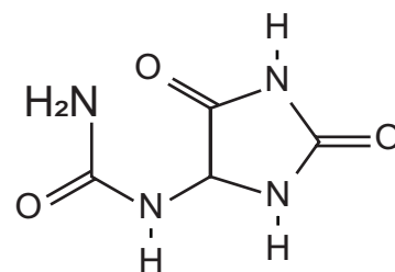
Allantoin Structure
