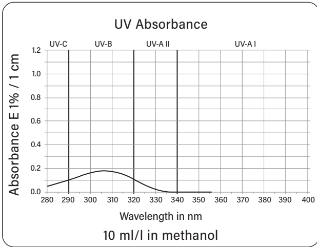
Ethylhexyl Salicylate
