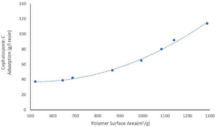
Figure 5. Adsorption isotherm of a Solution of Cephalosporin C (1% w/v Solution) vs. Surface Area (e.g. CT10 (>1200m²/g), LXA8302 (>1100 m²/g) and LXA84 (>700 m²/g)).
