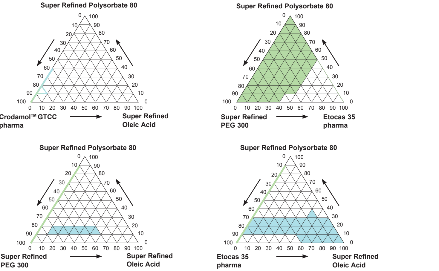
Figure 7: Phase diagrams of diluted, purified surfactants (Super Refined Polysorbate 20 or 80) co-surfactant (Etocas 35 pharma*), co-solvents (Super Refined PEG 300 and 400) and oils (Super Refined Oleic Acid or Crodamol GTCC pharma*) in distilled water. [ Green = SMEDDS (particle size of <50 nm); Light blue = SEDDS (particle size of 100-300 nm) ]
