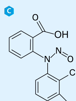
N-nitroso-mefenamic acid
