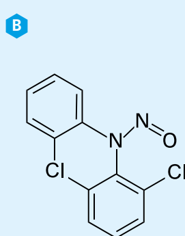
N-nitroso-diphenylamine
